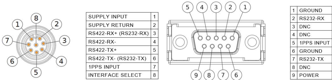
ADC Data Transfer Cable (Left) and RS232 Interface Connector (Right) Pinout
